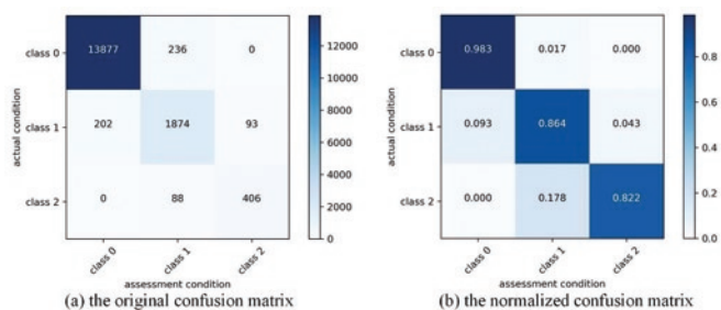
Fig. 15. Confusion matrixes with GAEM-II.2
