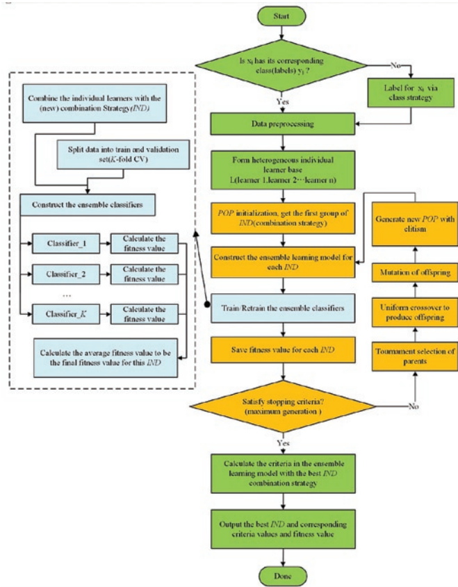
Fig. 1. Flowchart for GAEM
