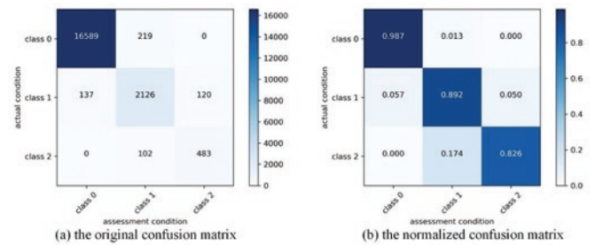
Fig. 16. Confusion matrixes with GAEM-II.3
