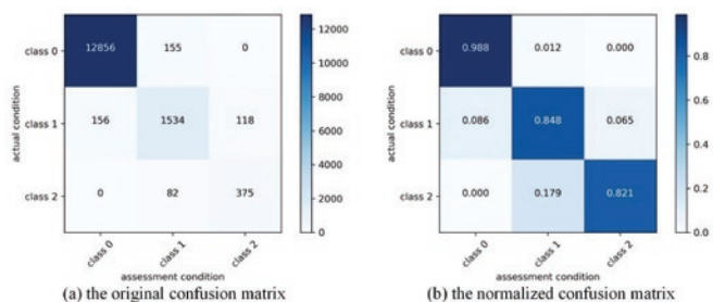
Fig. 14. Confusion matrixes with GAEM-II.1
