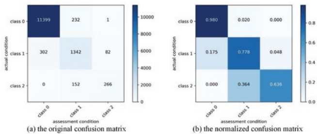
Fig. 10. Confusion matrixes with the common heterogeneous ensemble learning model
