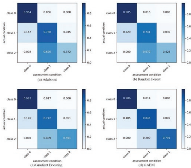
Fig. 12. The normalized confusion matrixes for Adaboost, Random Forest, Gradient Boosting and GAEM
